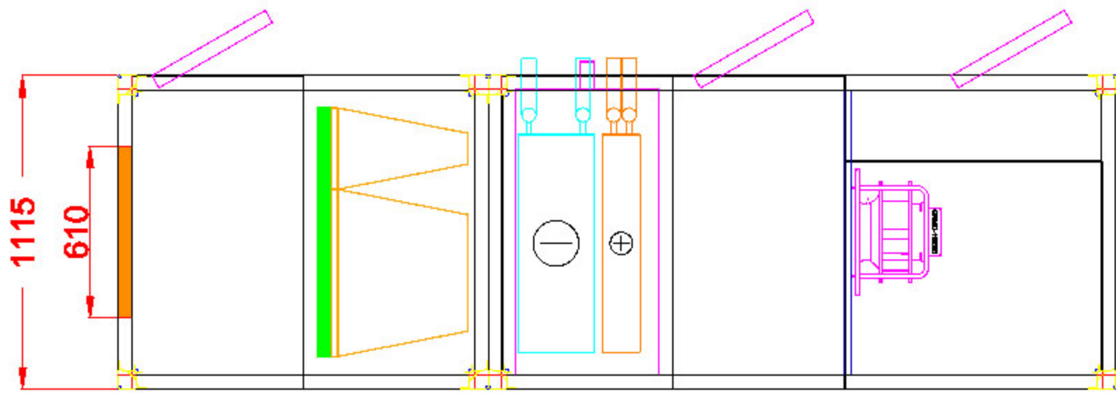
Top View
