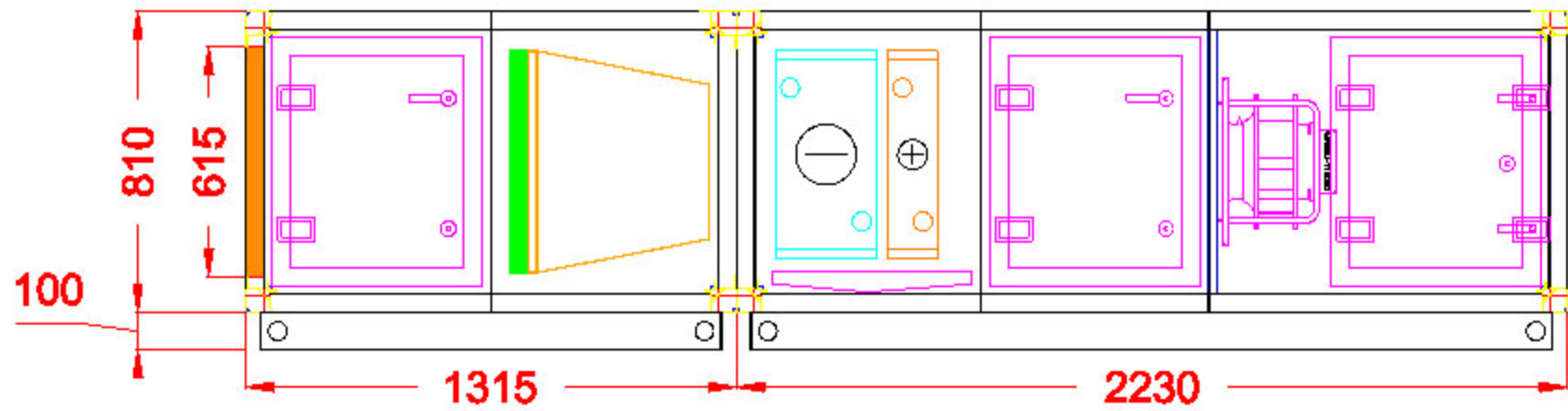
Right View
